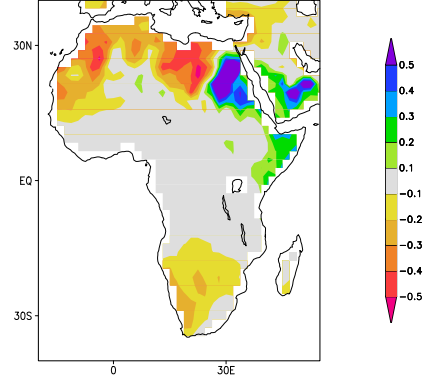
reldiff Jan-Dec gfdl 2.1 sresa1b pr 2036-2065 with Jan-Dec gfdl 2.1 sresa1b pr 1971-2000
