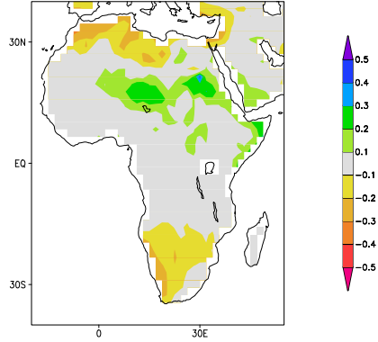
reldiff Jan-Dec gfdl 2.0 sresa1b pr 2036-2065 with Jan-Dec gfdl 2.0 20c3m pr 1971-2000
