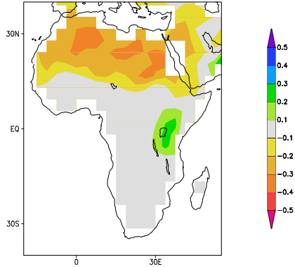
Fraction change in annual precipitation around 2050 compared with 1971-2000 in a few reasonable models
