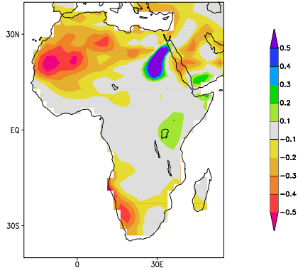
reldiff Jan-Dec cccma cgcm3.1 sresa1b pr 2036-2065 with Jan-Dec cccma cgcm3.1 sresa1b pr 1971-2000
