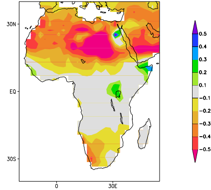
reldiff Jan-Dec hadgem1 sresa1b pr 2036-2065 with Jan-Dec hadgem1 sresa1b pr 1971-2000
