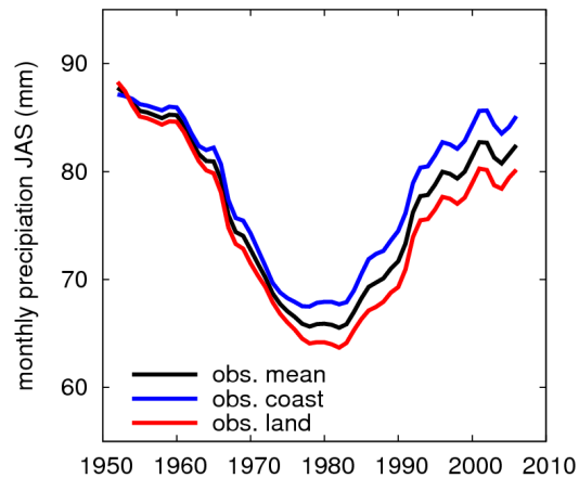
Figure 3. Time series of the 20-year moving average (smoothed with a 1-2-1 filter to remove high frequency noise) of mean, coastal and inland precipitation for late summer (July, August, September) in the Netherlands.
