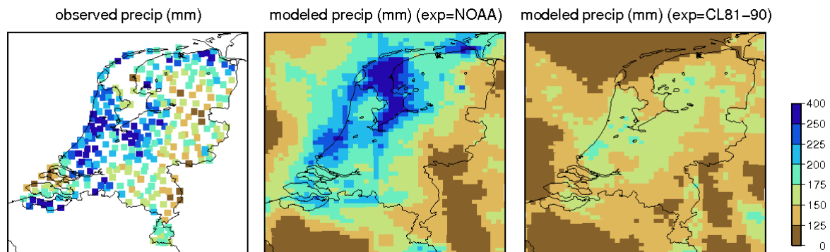
Figure 5. Observed precipitation amount (left), and modeled precipitation amount in experiments NOAA (middle) and CL81-90 (right panel) in August 2006 (mm).
