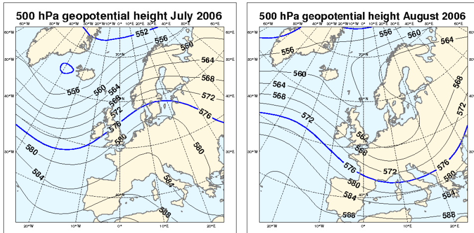
Figure 1. Synoptic situation during July (left) and August 2006 (right). Shown is the 500 hPa height obtained from the operational ECMWF analyses.
