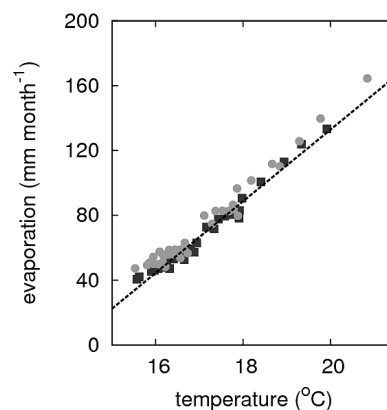
Figure 8. Relation between evaporation and sea surface temperature. A dot/square denotes the average of a zone (as defined in Figure 6). Black squares are averages over the month; grey dots are averages over the first 15 days of the month.
