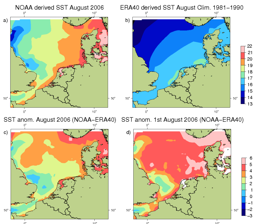
Figure 4. a) Observed SSTs inferred from NOAA satellite measurements for August 2006, b) ERA40 derived climatological SST for the period 1981-1990, c) anomaly August 2006 NOAA SST compared to the ERA40 1981-1990 climatology, and d) anomaly at the 1 st of August 2006.
