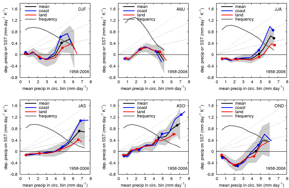
Figure 13. Regression coefficients of precipitation change (in \text{mm day}^{-1} per degree sea surface temperature) as a function of mean precipitation in each circulation bin. Results are plotted for the periods DJF, AMJ, JJA, JAS, ASO, OND, with particular emphasis on the late summer period. The grey band is the 10-90% uncertainty band in the estimation of the regression coefficient for the mean precipitation estimated by the bootstrap. Uncertainty bands for the coastal and inland zones are similar. The thin lines represent 1, 2, and 3 times the CC relation, respectively. The thick grey line is the number of days in each bin (divided by 1500).
