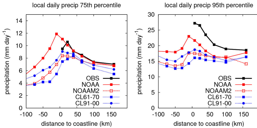
Figure 9. Extreme local (that is, station or grid box) daily precipitation amounts in August 2006 as a function of distance to the coast for the observations (black solid) and a selection of the model simulations (colored lines). Shown are the 75 (left) and 95th percentiles (right).
