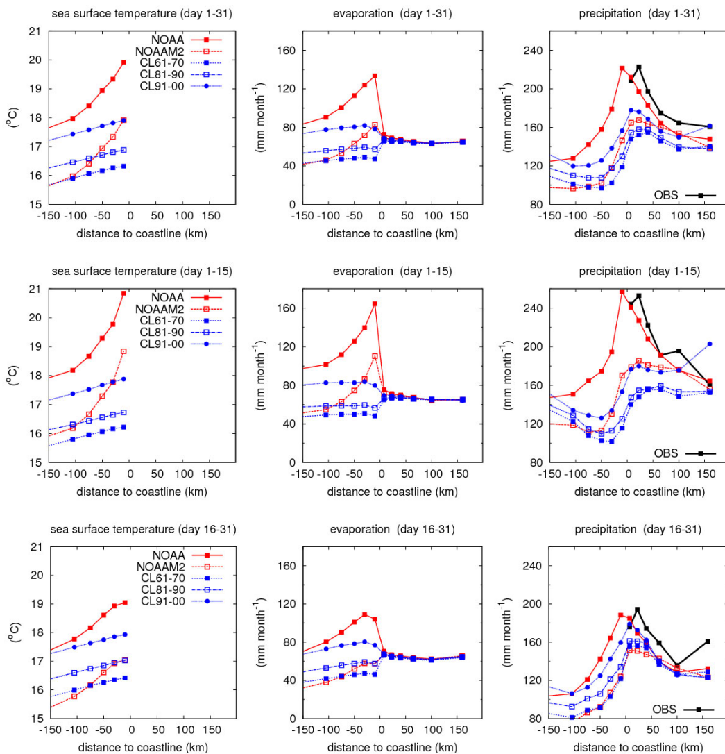
Figure 7. Sea surface temperature in ^{\circ}\text{C} (left), evaporation in \text{mm month}^{-1} (middle) and precipitation in \text{mm month}^{-1} (right-hand panels) as a function of distance to the coastline. The upper panels are based on the full month, the middle and the lower panel on the first half (day 1-15) and second half (day 16-31) of the month, respectively.
