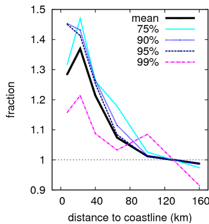
Figure 10. Observed mean and extreme precipitation amounts in August 2006 as a function of distance to the coast. Shown are relative differences (fraction) with respect to the observed average of the regions with distance of 80-120 and 120-200 km from the coastline.
