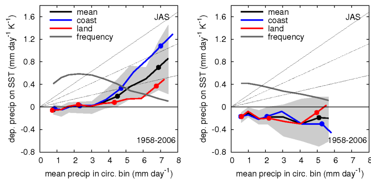
Figure 14. Same as Figure 13, but now only for JAS, and separated in days with a westerly flow ( G_w > 2 \text{ ms}^{-1} ) (left panel), and the remaining days ( G_w < 2 \text{ ms}^{-1} ) (right panel)
