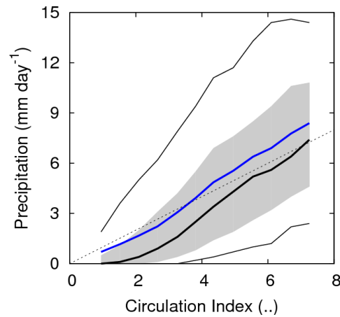
Figure 11. Mean precipitation in a circulation bin as a function of the average circulation index in the bin (blue line) for the period July, August, September (JAS). By construction it should be close to the 1-1 line (dotted line). The grey band denote the 25-75% range of the data, the solid lines the 10, 50, 90 th
