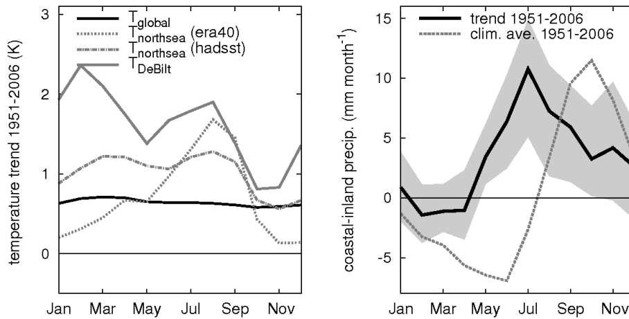
Figure 2. a) Temperature trends in the period 1951-2006. Shown is the trend in global mean near surface temperature ( T_{GL} ), the temperature at De Bilt, the sea surface temperature in the North Sea derived from ERA40 (only 1958-2006 period) and derived from HadSST. b) Precipitation difference between the coastal zone and the inland zone as a function of month. Shown is the climatology over the period 1951-2006 (dashed line) and the trend over this period (change in \text{mm month}^{-1} per 55 year) (thick solid line, with the grey band indicating the 10-90% uncertainty range). Both plots are based on overlapping 3-month periods, e.g. Jul refers to the average of June, July, and August.
