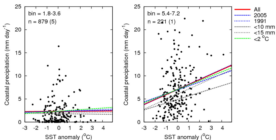
Figure 12. Coastal precipitation amounts versus the SST anomaly for two circulation bins (left relatively dry circulation, right wet circulation). Different fits to a number of selections of the data are shown; all: all days 1958-2006; 2005 (1991): all days from 1958 until 2005 (1991) (inclusive); <10 (15) mm: days with precipitation below 10 (15) mm day -1 ; <2K days with SST anomalies between -2 and +2 K.
