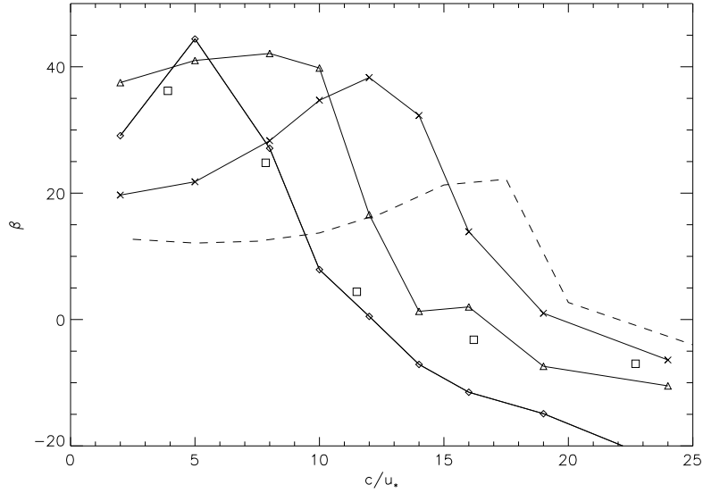
FIGURE 9. Growth rate as a function of wave age: —, low- Re model for Re = 260 ( \diamond ), Re = 1000 ( \Delta ) and Re = 4000 ( \times ); - - -, high- Re model ( kz_0 = 10^{-4} ); \square , direct numerical simulation at Re = 260 by Sullivan et al. (1999).
