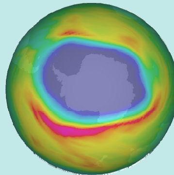
The ozone hole over the Antarctic region on 5 October, 2006
