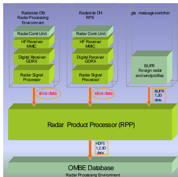
Figure 2 The radar production chain
