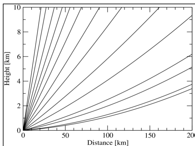
Figure 3 The Volume Coverage Pattern
