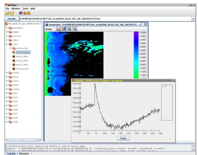
Figure 4 Transmitted power as metadata to moment data
