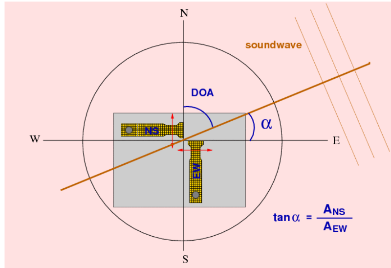
Fig. 3: A schematic of a measurement station defining the angles used. The thin, two-headed red arrows show the sensitive direction of the velocity probes. The DOA is the angle of the incoming sound wave with the North.
