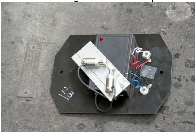
Fig. 1: A photograph of a measurement station. The Microflown probes are oriented perpendicular and are mounted on the electronic box. The coloured wires lead to the connectors for the signal cables. A probe is 1/2 inch wide.
