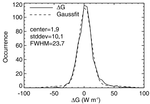
Figure 4. Distribution of the differences between simulated and measured global irradiances ( \Delta G ) for all the selected cases and the Gaussian fit. The unit for the center, standard deviation, and full width half maximum (FWHM) is \text{W/m}^2 .
