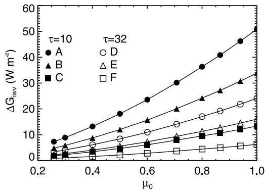
Figure 8. Sensitivity of the global irradiance to integrated water vapor column (IWV) as a function of \mu_0 . \Delta G_{\text{iwv}} is the difference between the global irradiance calculated with IWV = 0.5 (circles labeled A and D), 1 (triangles labeled B and E), and 2 cm (squares labeled C and F) and the global irradiance calculated with IWV = 2.96 cm, for cloud optical thickness of 10 (symbols A–C) and 32 (symbols D–F). r_e = 8 \mu\text{m} .
