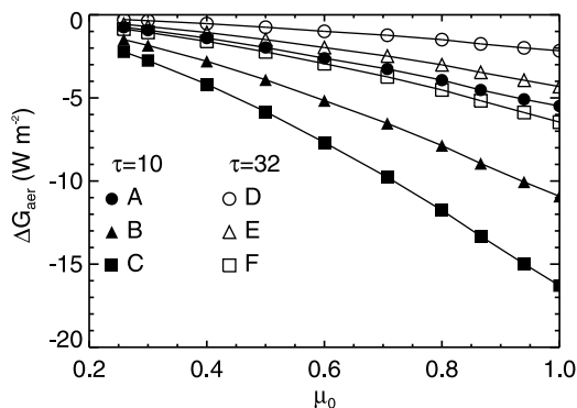
Figure 7. Sensitivity of global irradiance to AOT as a function of \mu_0 . \Delta G_{\text{aer}} is the difference between the global irradiance calculated with AOT = 0.1 (circles labeled A and D), 0.2 (triangles labeled B and E), and 0.3 (squares labeled C and F) and the global irradiance calculated with AOT = 0, for cloud optical thickness of 10 (symbols A–C) and 32 (symbols D–F). r_e = 8 \mu\text{m} .
