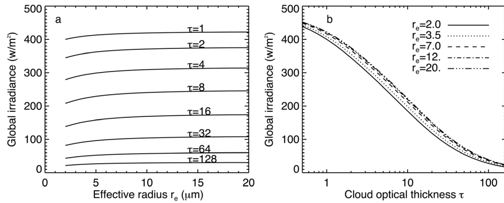
Figure 6. (a) Global irradiance at the surface varied as a function of effective radius ( r_e ) for different cloud optical thicknesses ( \tau ) for water clouds. (b) Global irradiance at the surface varied as a function of \tau , for different values of r_e (in \mu\text{m} ). In both plots, \mu_0 = 0.5 .
