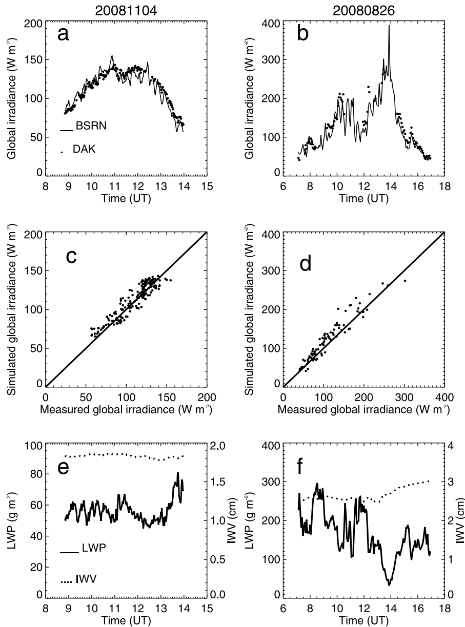
Figure 1. Results for (a, c, e) 4 November and (b, d, f) 26 August 2008. Figures 1a and 1b show the global irradiances from BSRN measurements at Cabauw (solid line) and the DAK simulations (solid circles). Figures 1c and 1d show scatterplots of simulated versus measured global irradiances. The solid line indicates the one-to-one line. Figures 1e and 1f show the cloud liquid water paths (solid line, left y axis) and integrated water vapor columns (dotted line, right y axis).
