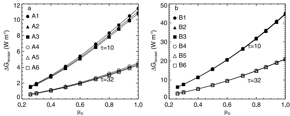
Figure 9. Sensitivity of the global irradiance to a simultaneous variation of IWV and AOT. (a) \Delta G_{\text{iwvaer}} is the difference in global irradiance between AOT = 0 and 0.2 for cases with IWV = 0.5 (circles labeled A1 and A4), 2 (triangles labeled A2 and A5), and 4 (squares labeled A3 and A6) cm. (b) \Delta G_{\text{iwvaer}} is the difference in global irradiance between IWV = 1 and 4 cm for cases with AOT = 0 (circles labeled B1 and B4), 0.1 (triangles labeled B2 and B5), and 0.2 (squares labeled B3 and B6). Cloud optical thickness is 10 and 32. r_c = 8 \mu\text{m} .
