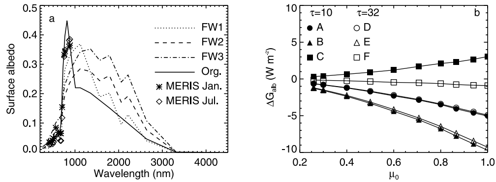
Figure 10. (a) The grass reflectance spectra FW1, FW2, and FW3; the surface albedo spectrum used to generate the LUTs (“Org.”); and the MERIS surface albedo climatology for Cabauw in January and July. (b) Sensitivity of the global irradiance to surface albedo as a function of \mu_0 . \Delta G_{\text{alb}} is the difference between the global irradiance calculated with grass reflectance spectrum FW1 (circles labeled A and D), FW2 (triangles labeled B and E), and FW3 (squares labeled C and F) and the global irradiance calculated from the reference LUT, for cloud optical thickness of 10 (symbols A–C) and 32 (symbols D–F). r_c = 8 \mu\text{m} .
