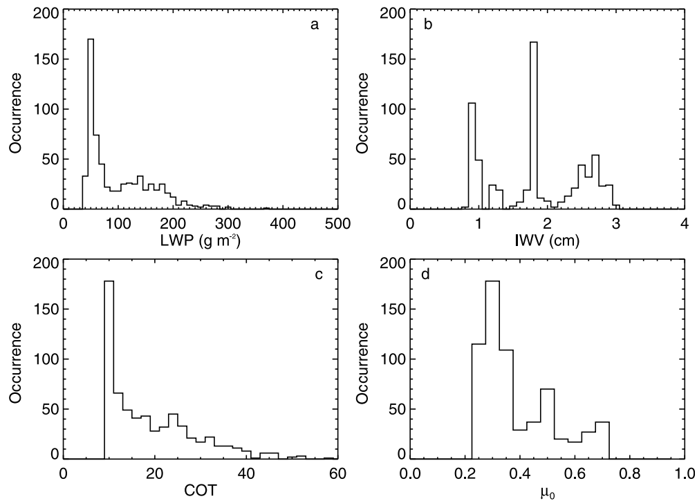
Figure 2. Histograms of (a) cloud liquid water path (LWP), (b) integrated water vapor column (IWV), (c) cloud optical thickness (COT), and (d) cosine of solar zenith angle ( \mu_0 ) for all the cloud cases.
