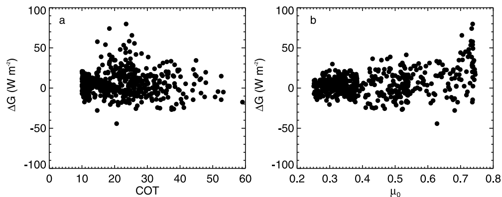
Figure 5. The differences between the simulated and measured global irradiances ( \Delta G ) as a function of (a) cloud optical thickness (COT) and (b) cosine of solar zenith angle ( \mu_0 ) for all the selected cases.
