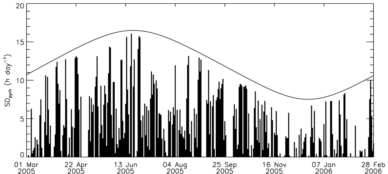
FIG. 3. Pyrheliometric daily sunshine duration ( SD_{\text{pyrh}} ; \text{h day}^{-1} ) for Cabauw (Fig. 1) for the period March 2005–February 2006. The values are obtained from summation of sunshine seconds determined by means of application of the WMO threshold of 120 \text{ W m}^{-2} for the direct solar irradiance. Also shown is the day length (solid line), which is defined as the time of the day for which \mu_0 > 0 ( \mu_0 was not corrected for atmospheric refraction).
