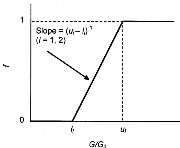
FIG. 2. Schematic representation of the correlation algorithm for the estimation of sunshine duration from global irradiance measurements [see Eq. (4)]. On the vertical axis the fractional sunshine duration ( f ) is given; on the horizontal axis the normalized global irradiance is given ( G/G_0 ). The lower limit for G/G_0 below which f = 0 is indicated by l_i ; the upper limit for G/G_0 above which f = 1 is indicated by u_i . The index i indicates a separation for \mu_0 in two intervals: \mu_0 < 0.3 and \mu_0 \geq 0.3 .
