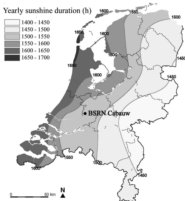
FIG. 1. Distribution of yearly sunshine duration ( \text{h yr}^{-1} ) for the Netherlands, averaged over the period 1971–2000 (Heijboer and Nellesstijn 2002). Until 1 Oct 1992 sunshine duration has been determined by means of the Campbell–Stokes sunshine recorder at about 25 stations. From that date onward, sunshine duration has been estimated from global irradiance according to an adjusted version of the Slob algorithm (see sections 2 and 5). The BSRN site of Cabauw is indicated. The analysis presented here is based on measurements of direct and global irradiance made at this site.
