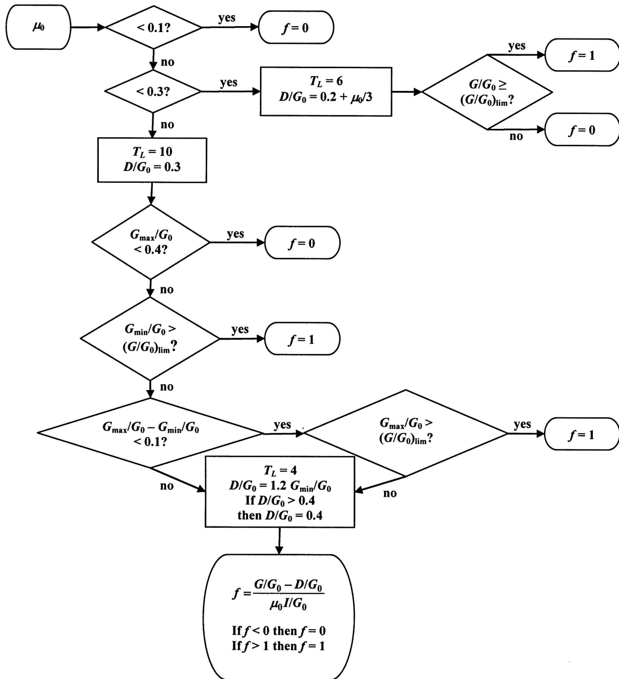
FIG. A1. Flow diagram of the Slob algorithm. The algorithm has been designed by Slob and Monna (1991) and is based on the use of mean, minimum, and maximum values of the measured global irradiance over a 10-min interval to estimate the fractional sunshine duration ( f ) for this interval. Furthermore, the algorithm relies on parameterized estimates of the direct and diffuse irradiance under cloudless conditions.
