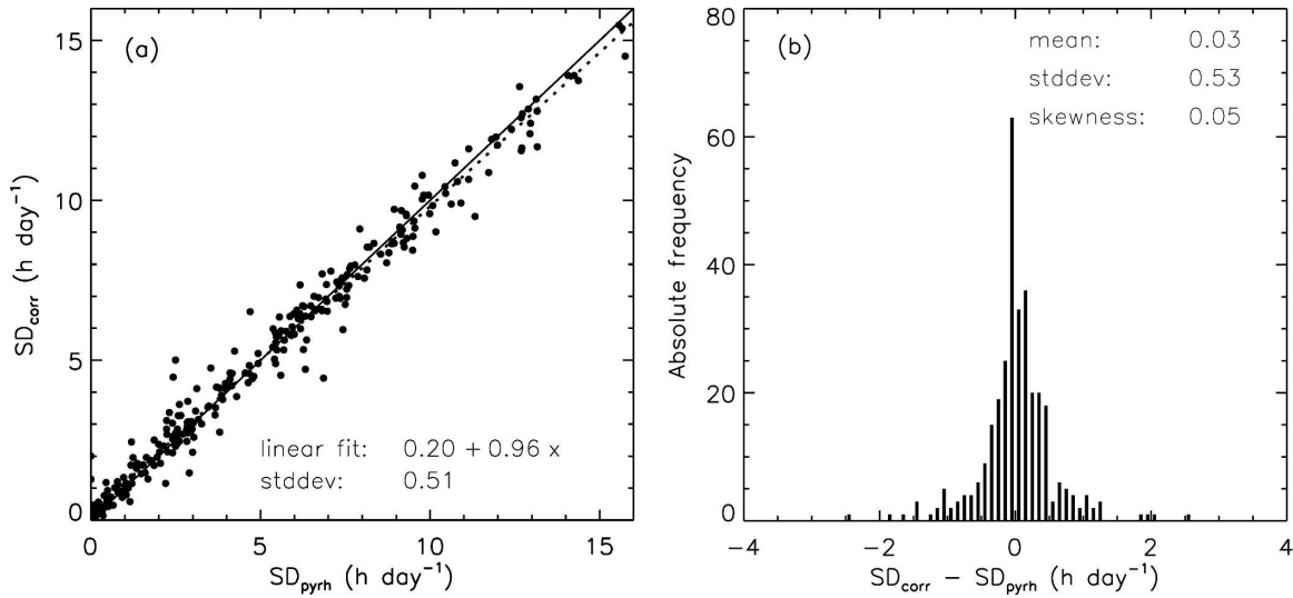
FIG. 6. (a) Daily sunshine durations ( h \text{ day}^{-1} ) as calculated by means of the correlation algorithm ( SD_{corr} ) vs corresponding pyr heliometric sunshine durations ( SD_{pyrh} ). Also shown are the 1:1 line (solid) and a linear fit through the data (dotted line). (b) Absolute frequency distribution of SD_{corr} - SD_{pyrh} ( h \text{ day}^{-1} ).
