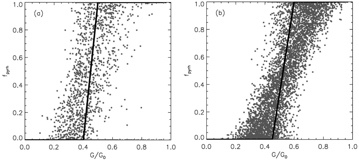
FIG. 5. Measurements (gray points) of the pyrheliometric fractional SD ( f_{\text{pyrh}} ) vs 10-min mean measurements of the normalized global irradiance ( G/G_0 ) for (a) \mu_0 < 0.3 and (b) \mu_0 \geq 0.3 . The solid lines indicate the fits used for the correlation algorithm [Eqs. (4) and Fig. 2] to directly estimate SD from global irradiance measurements. The fitted parameters for G/G_0 are l_1 = 0.4 , u_1 = 0.5 , l_2 = 0.45 , and u_2 = 0.6 .
