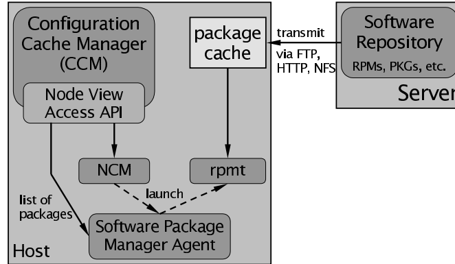
Figure 4. Components for managing software installation
