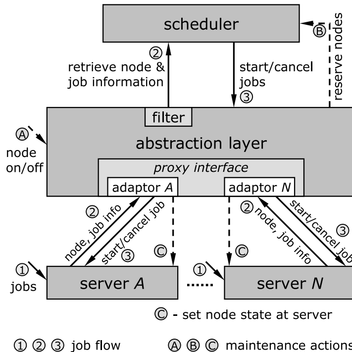
Figure 9. Support for job management and maintenance actions across several clusters.
