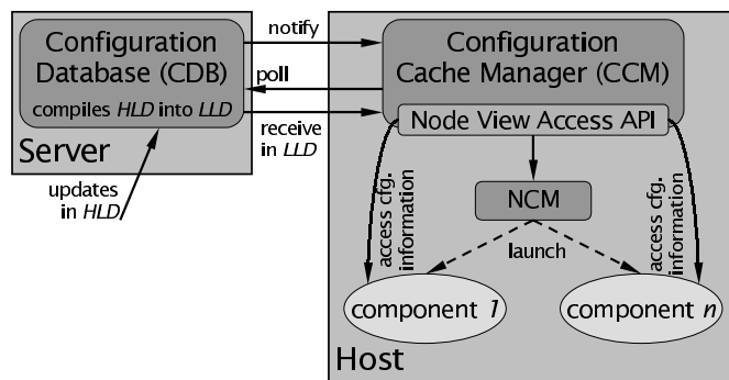
Figure 2. Components for managing configuration information
