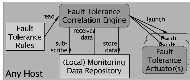
Figure 6. Components of the fault tolerance system
