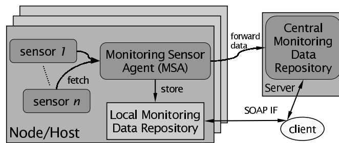
Figure 5. The monitoring system consisting of sensors, a sensor controller, a local and a central monitoring data repository.
